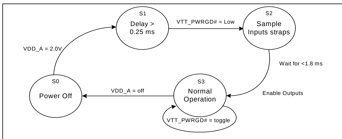
Figure 10. VTT_PWRGD# Timing Diagram
