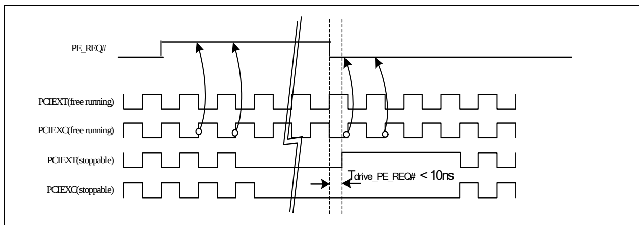
Figure 9. CLKREQ# De-Assertion
